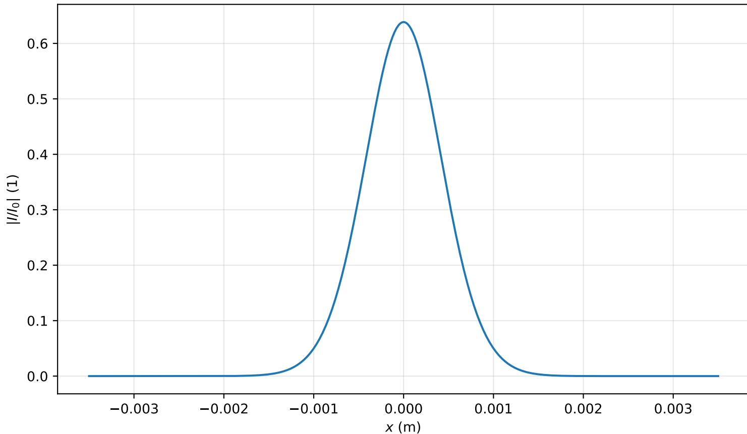
Intensity profile I(x, y = 0, z = 1.831m)/I_0 , P_{in}=0.2P_{cr} , artificial time
